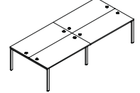
BG044 / VBG044 3200/1400/758
